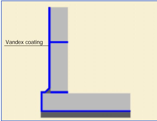
External waterproofing
