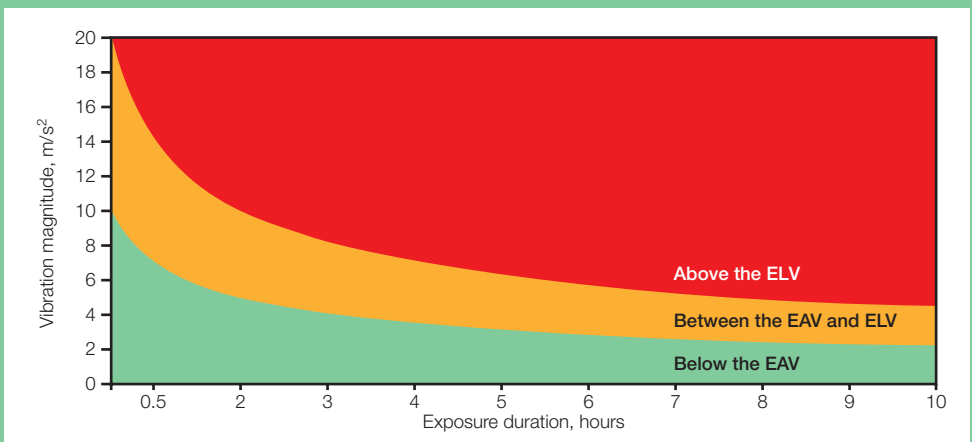
Figure 1 How vibration level and duration affect exposure
